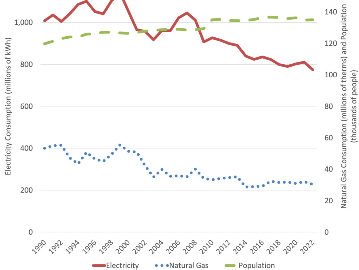
Figure 10. Electricity consumption, natural gas consumption, and population in Humboldt County, 1990 to 2022 (Data sources: CEC, 2024a; CEC, 2025a; FRED, 2025).
