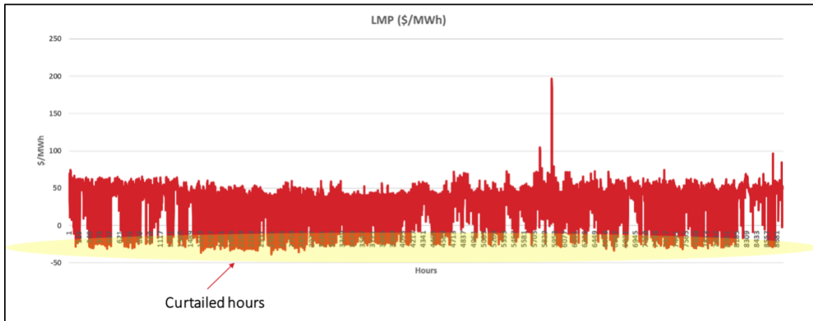
Figure 4-4. LMPs at the Humboldt Substation for the 144 MW OSW Farm
