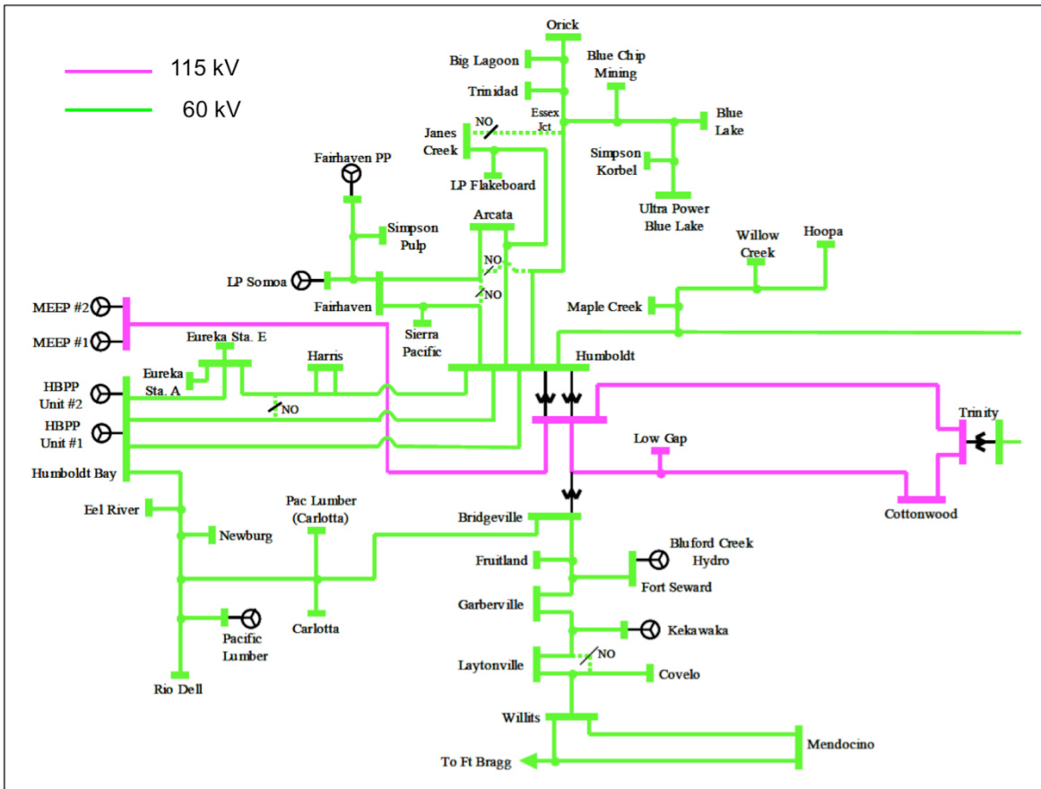
Figure 1.4: Humboldt Area Electricity Transmission Schematic
