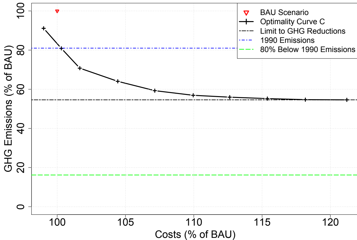
Figure 3.2: Optimality Curve (Curve C) - Minimize Emissions with Various Cost Ceilings
