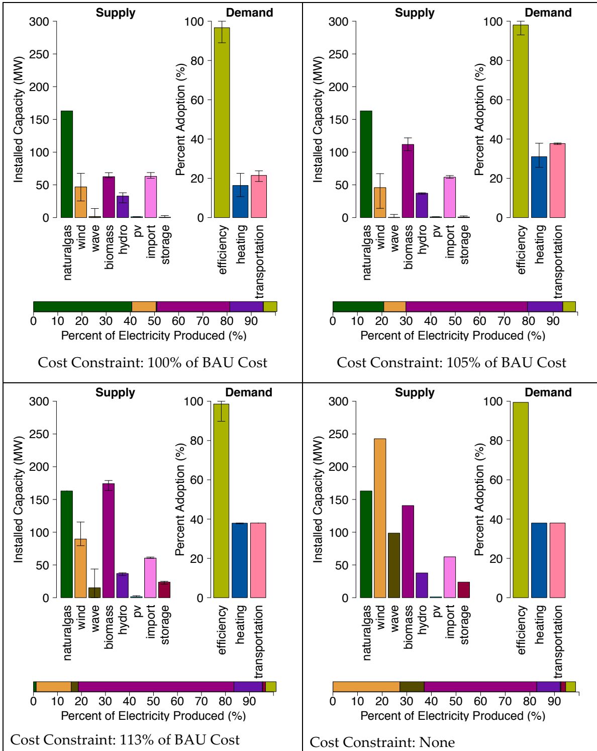
Figure 3.3: Portfolios from Optimality Curve C
