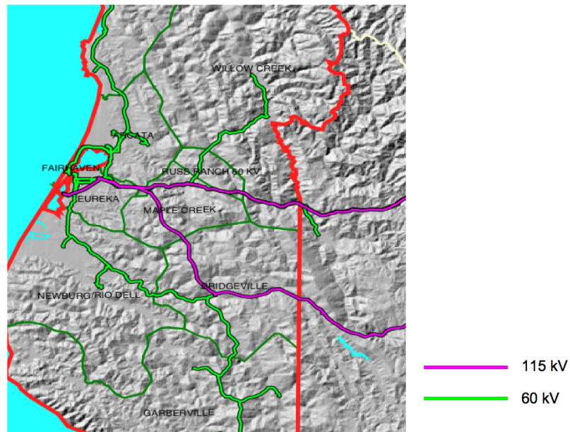
Figure 1.5: Humboldt Area Electricity Transmission Map
