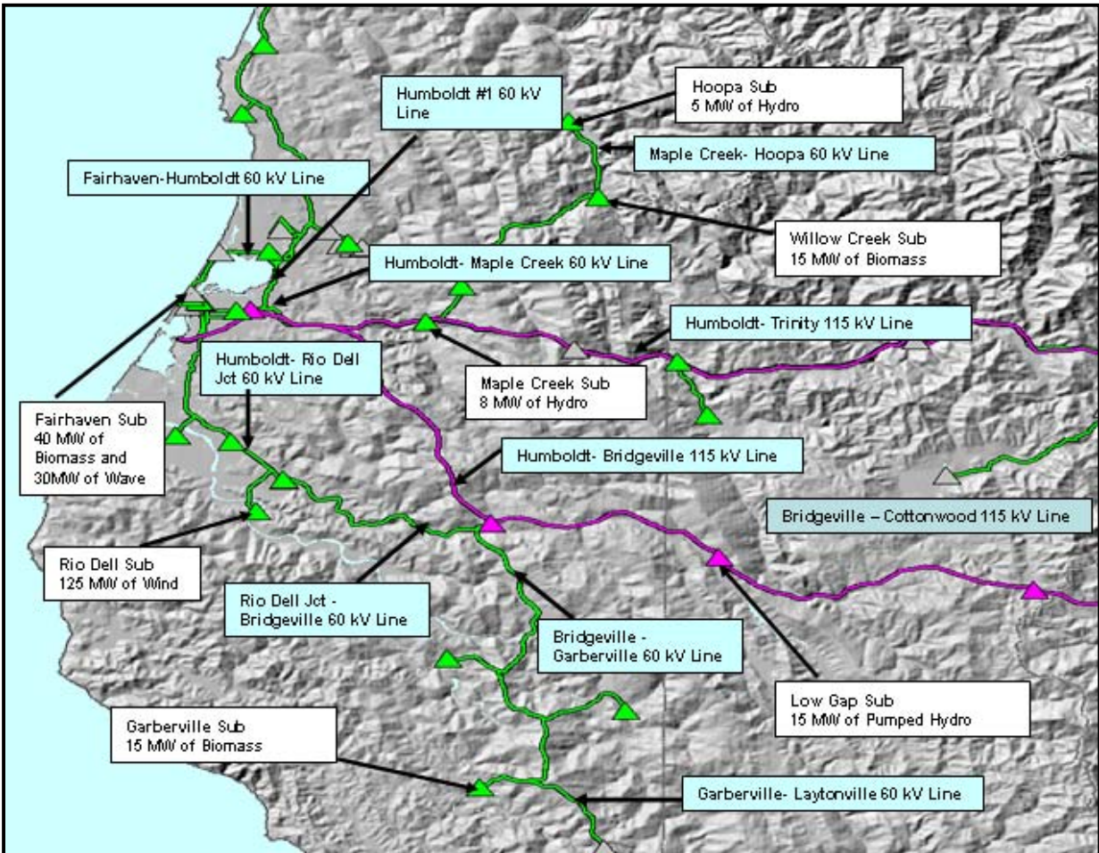
Figure 2.3: Locations of New Generation Facilities and Interconnection Points
