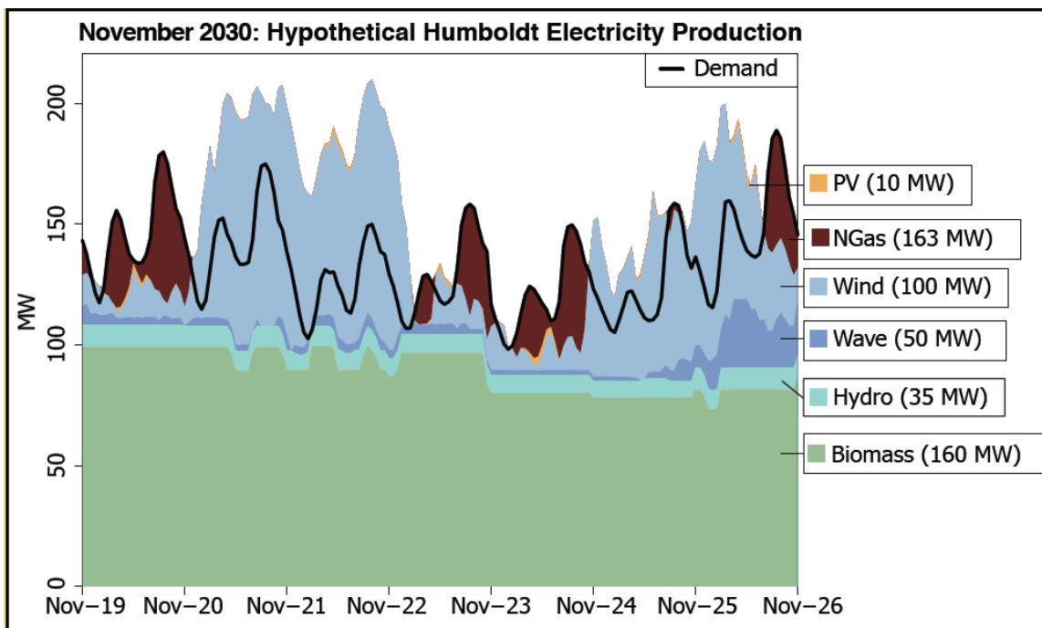
Figure 3.1: Example Hourly Supply and Demand Profile from REPOP Model
