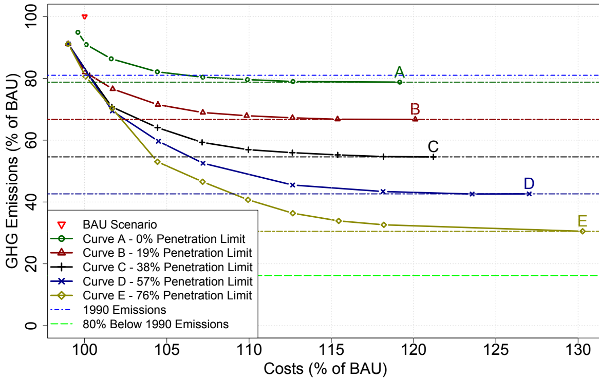
Figure 3.4: Optimality Curves With Varying Limits on the Penetration of Electric Vehicles and Heat Pumps
